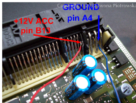
Connecting emulator to ECU
