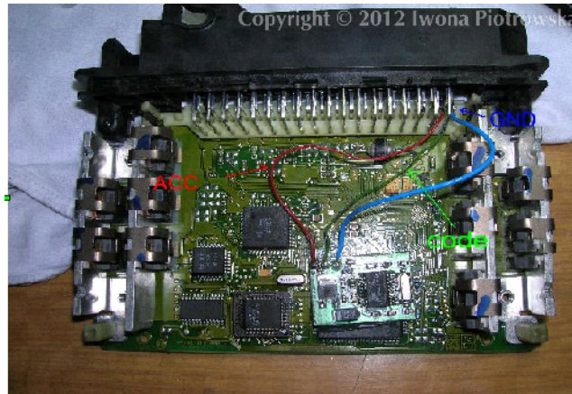
Connecting emulator to ECU
