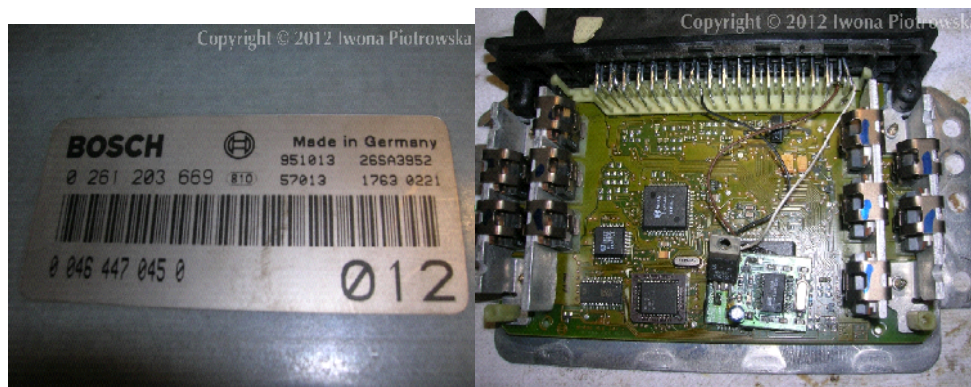
Connecting emulator to ECU
