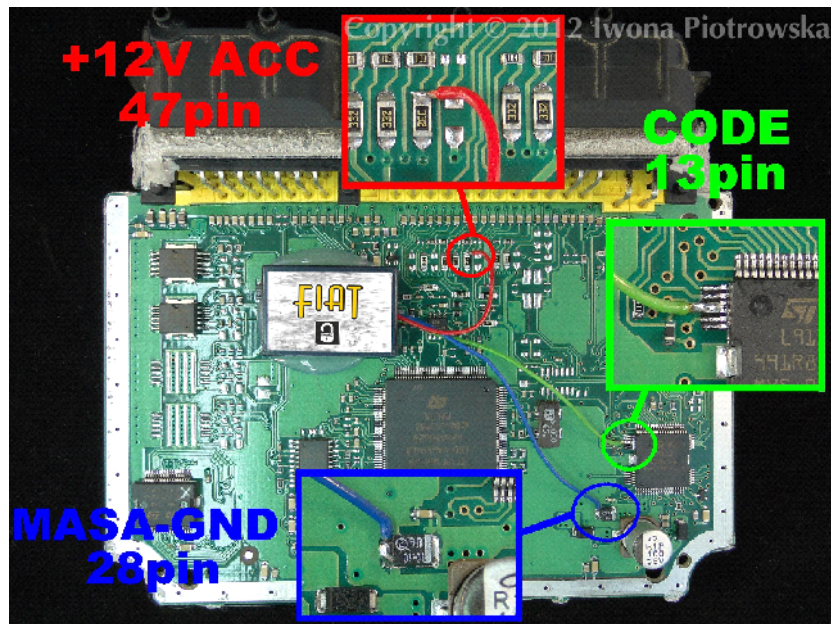
Connecting emulator to ECU
